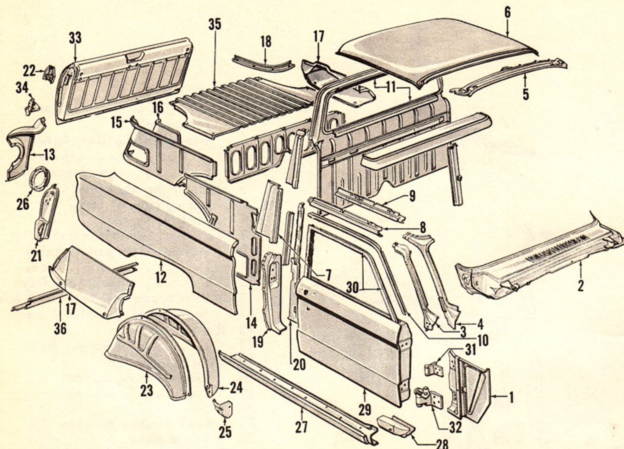
RANCHERO BODY PANELS
