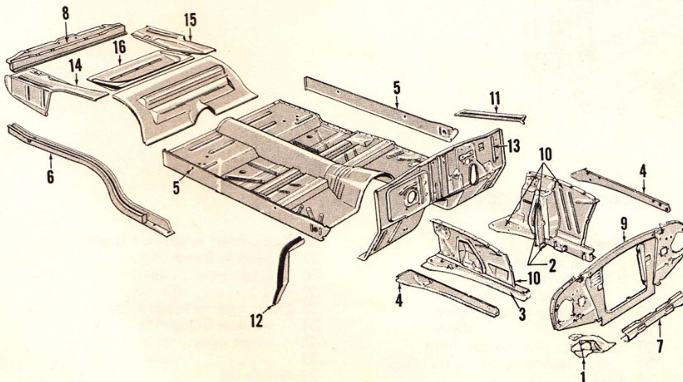
UNDERBODY PARTS
