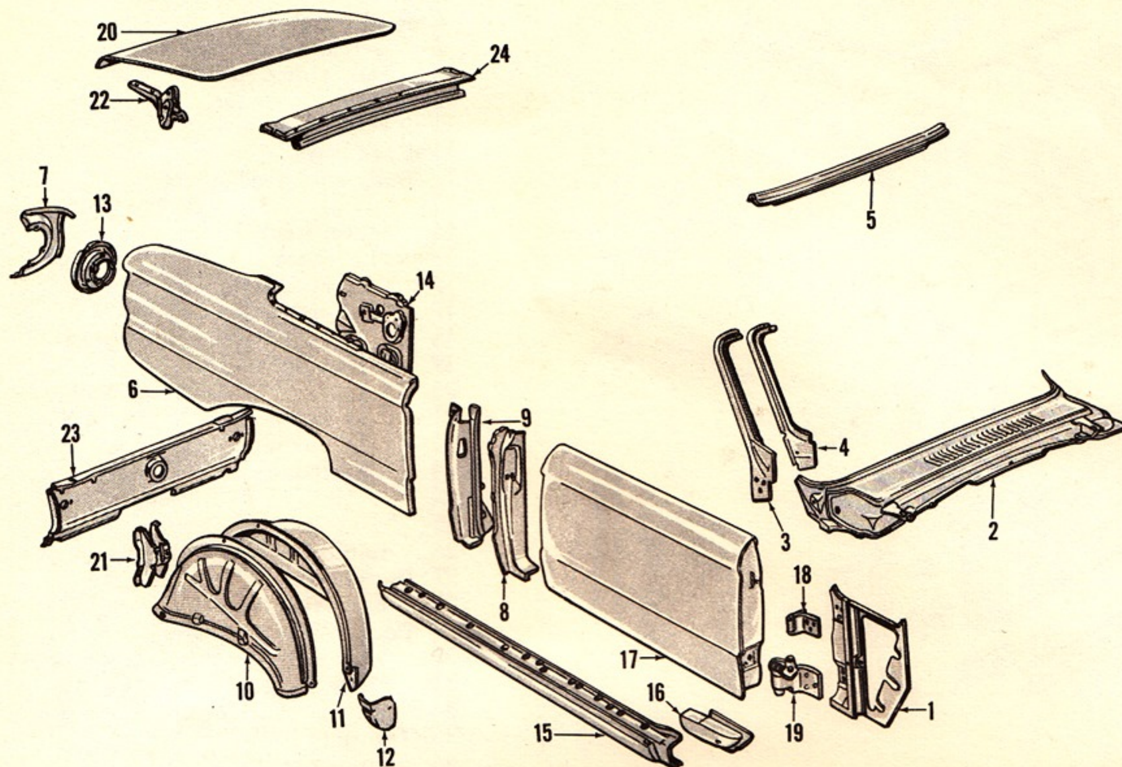
CONVERTIBLE BODY PANELS
