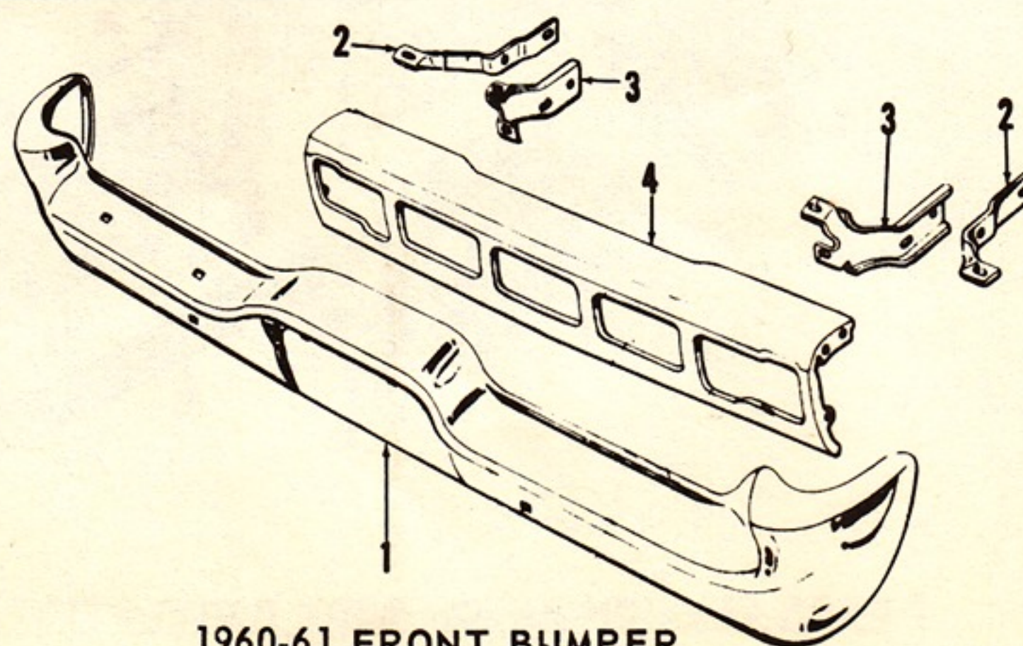
1960-61 FRONT BUMPER
