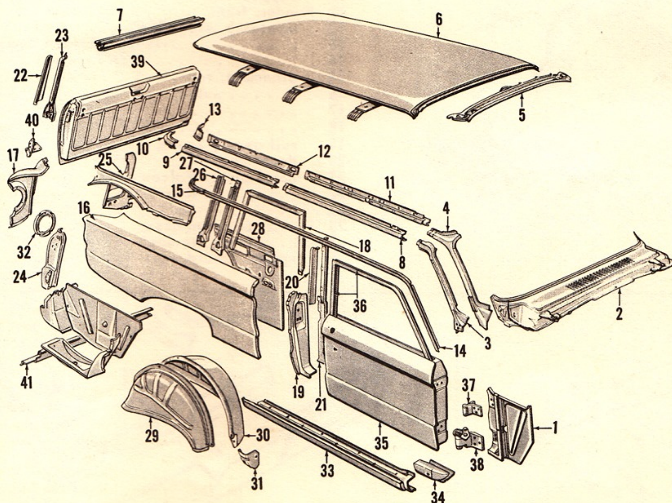
2-DOOR STATION WAGON BODY PANELS (TYPICAL OF SEDAN DELIVERY)
